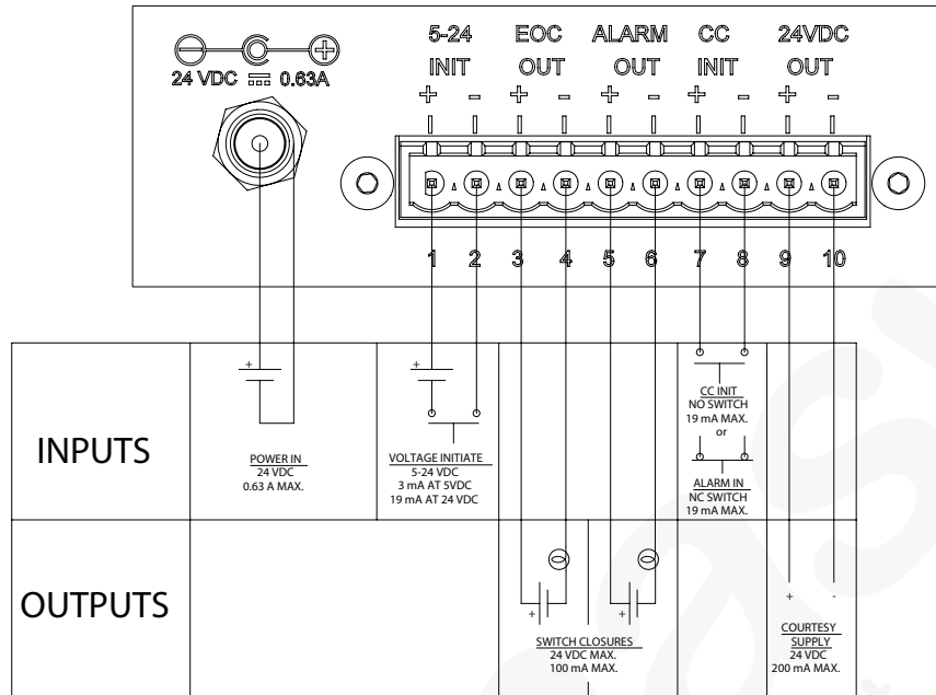
I/O External Wiring Diagram
