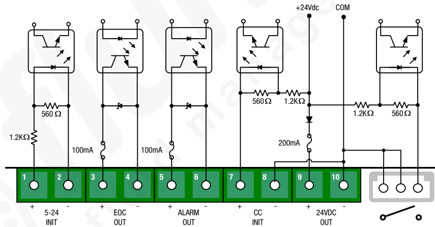
I/O Electrical Schematic
